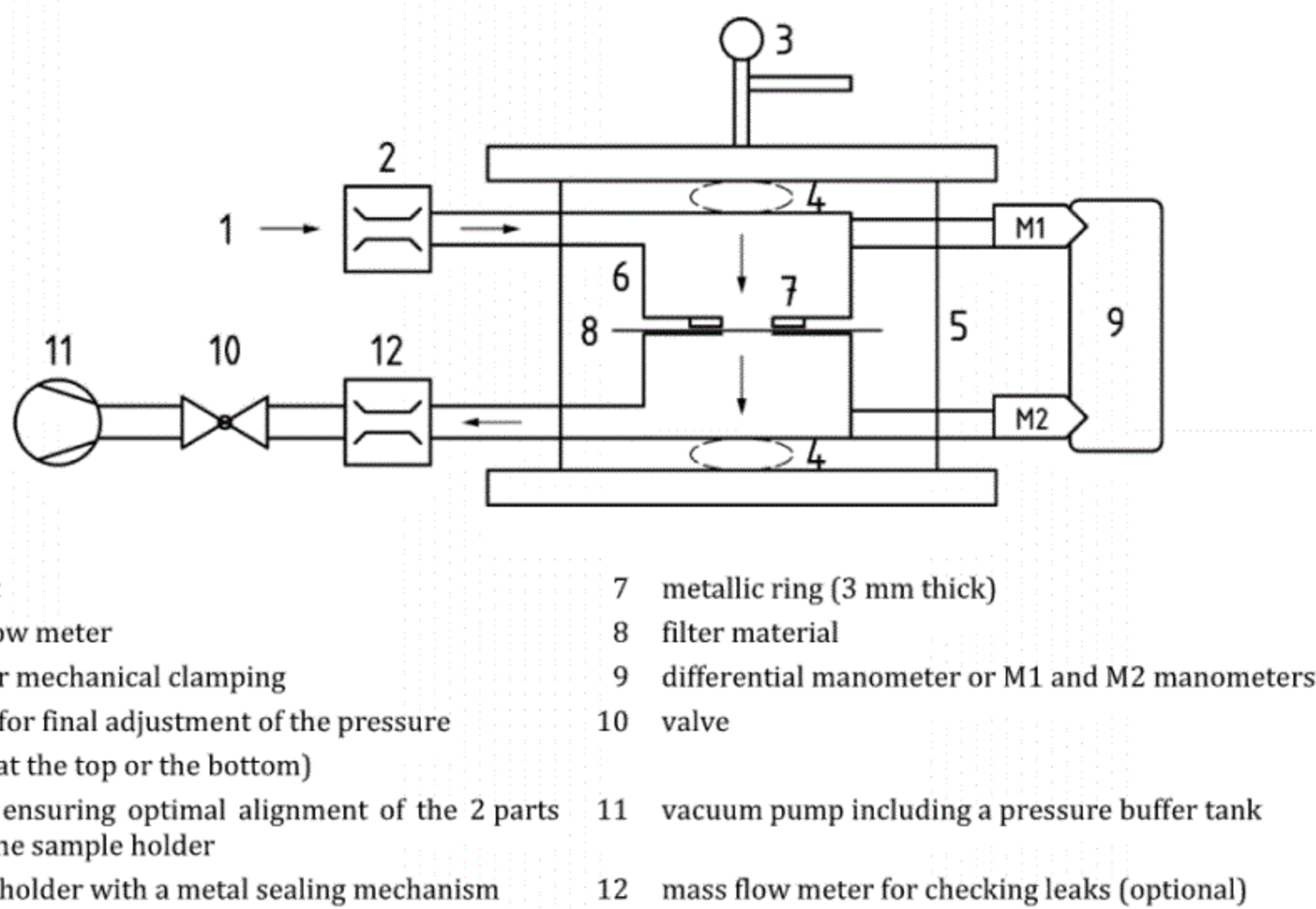
Figure C.1 — Test apparatus for measuring differential pressure
